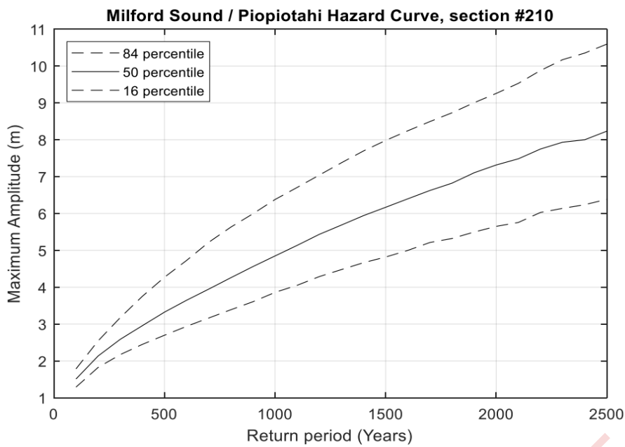
Figure 5: Return period of different tsunami waves heights at Milford Sound Piopiotahi (source: GNS science 2021 National Tsunami Model).
