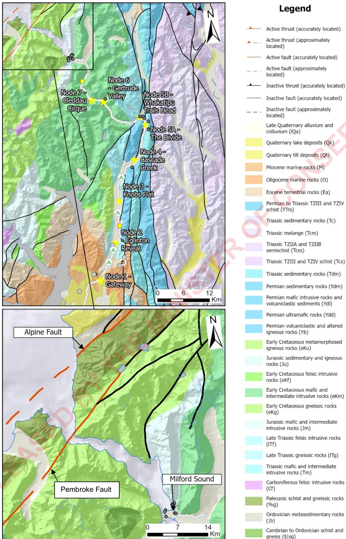
Figure 3: The GNS 1:1M Geological Map of the study area with a zoomed in inset map of Milford sound and the Alpine Fault (bottom).
