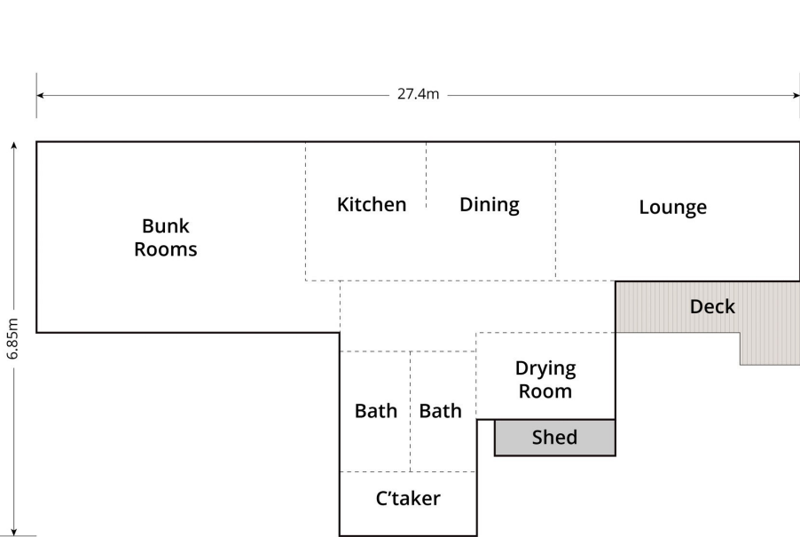
Current Floor Plan Approx Area 235m 2
