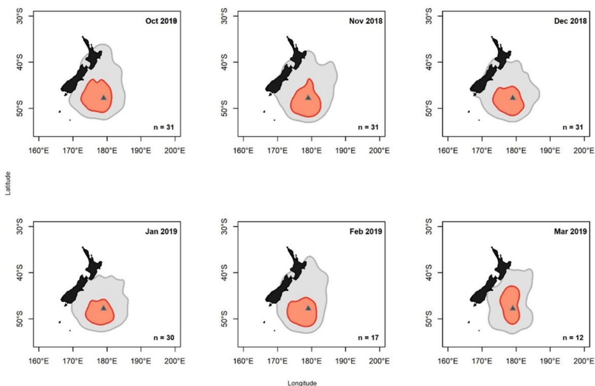
Figure 3-1: Kernel density utilisation distributions (UDs) for breeding Salvin's albatrosses at the Bounty Islands, 2018-2019, based on GLS data. The 50% UD (red) and 95% (grey) are shown, and the colony location is represented by the dark grey triangle.
