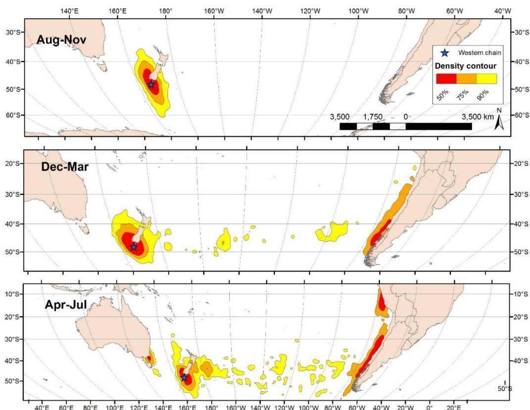
Figure 4-1: Kernel density utilisation distributions (UDs) for breeding Salvin's albatrosses at the Western Chain, Snares Islands, 2008-2009, based on GLS data. The 50% (red), 75% UD (orange) and 90% UD (yellow) are shown, and the colony location is represented by the blue star. Number of birds = 24. Thompson et al. 2014.
