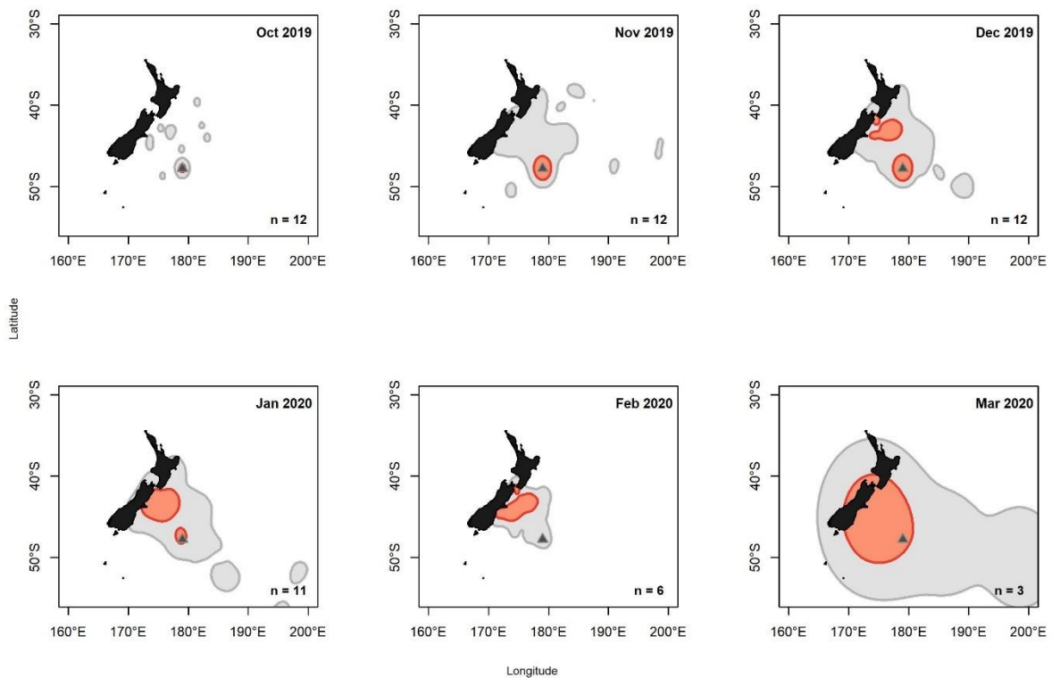
Figure 3-4: Kernel density utilisation distributions (UDs) for breeding Salvin's albatrosses at the Bounty Islands, 2019-2020, based on PTT data. The 50% UD (red) and 95% UD (grey) are shown, and the colony is represented by the dark grey triangle. Number of devices is indicated at the lower right of each plot.
