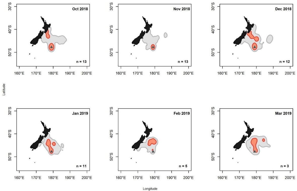
Figure 3-2: Kernel density utilisation distributions (UDs) for breeding Salvin's albatrosses at the Bounty Islands, 2018-2019, based on GPS data. The 50% UD (red) and 95% UD (grey) are shown, and the colony is represented by the dark grey triangle. Number of active devices is indicated at the lower right of each plot.
