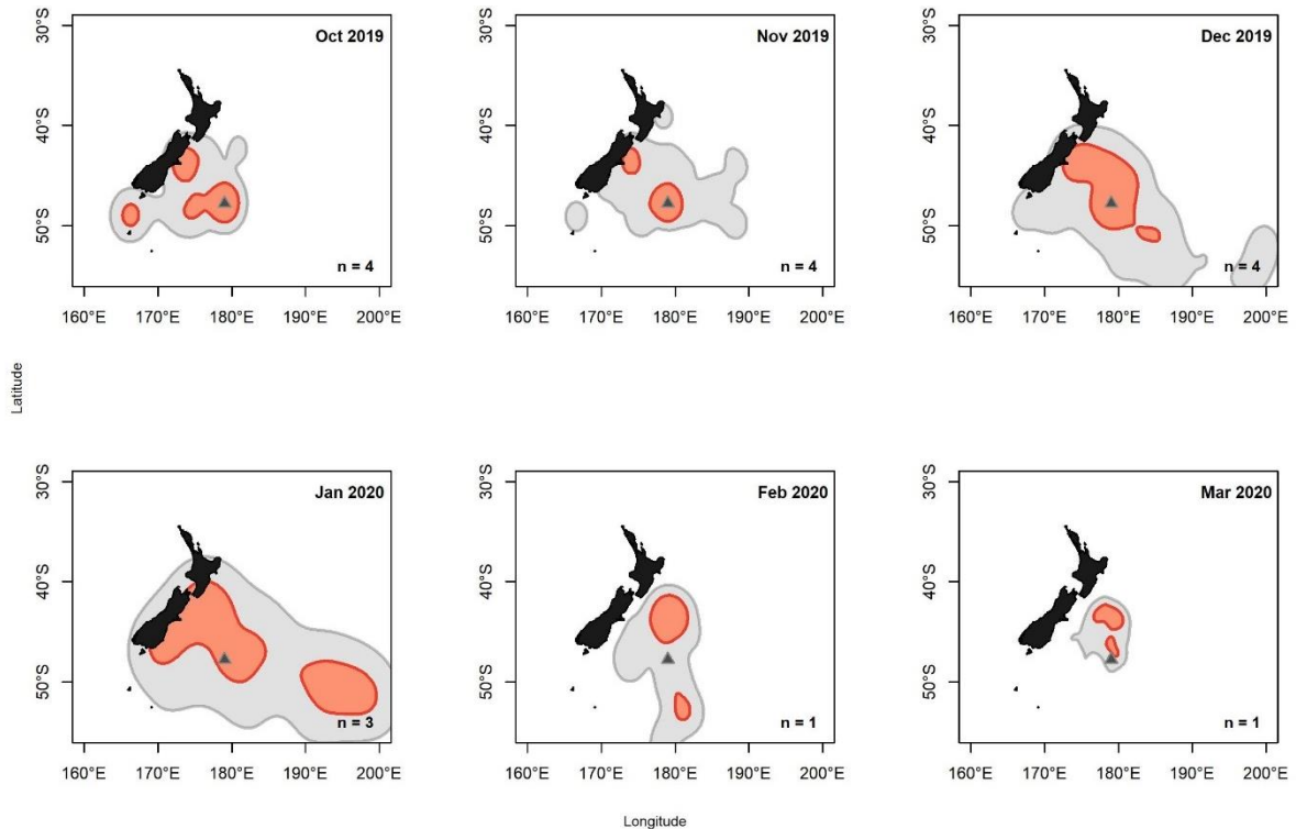
Figure 3-3: Kernel density utilisation distributions (UDs) for breeding Salvin's albatrosses at the Bounty Islands, 2019-2020, based on GPS data. The 50% UD (red) and 95% UD (grey) are shown, and the colony location is represented by the dark grey triangle. Number of active devices is indicated at the lower right of each plot.
