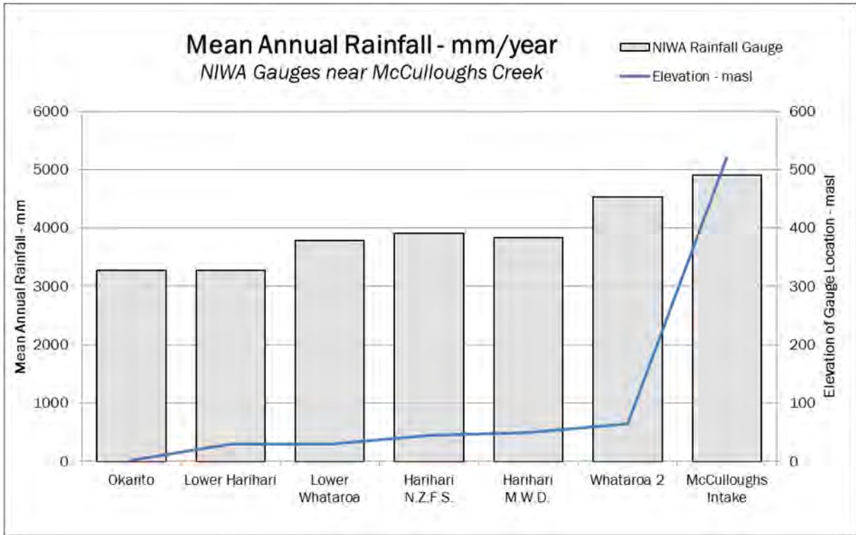
Figure 25 – Mean Annual Rainfall at Gauges near McCulloughs Creek Intake
