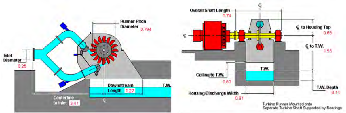
Figure 9 - Turbine and generator dimensions
