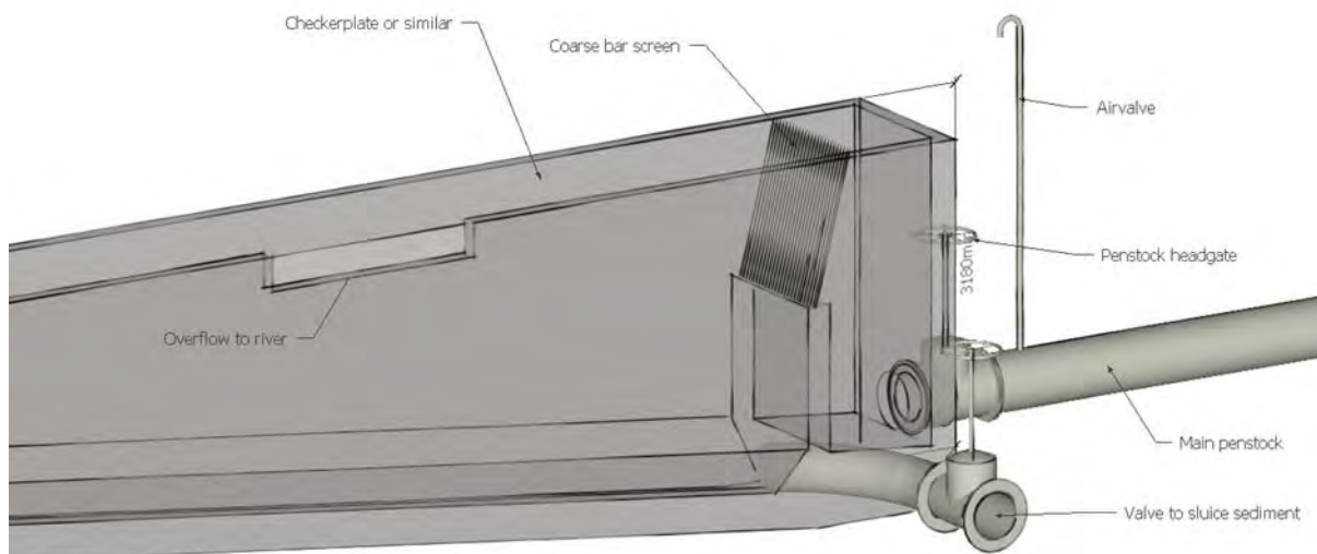
Figure 7 – Desander
