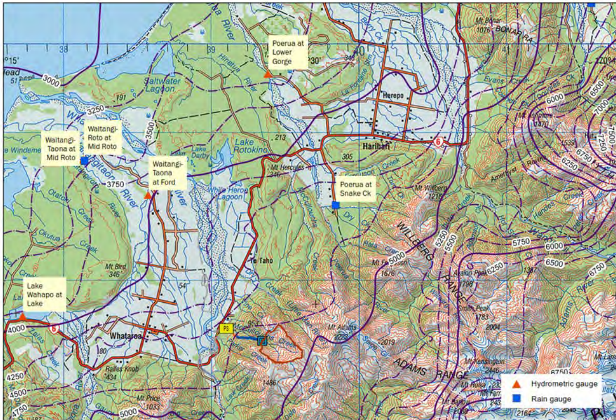
Figure 26 – Map showing NIWA rain gauges, hydrometric gauges and rainfall isohyets
