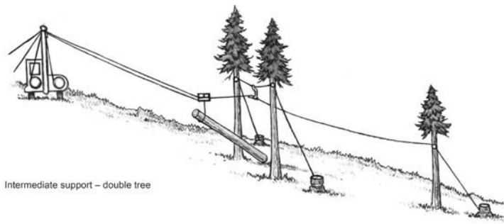
Figure 14 – Intermediate support example
