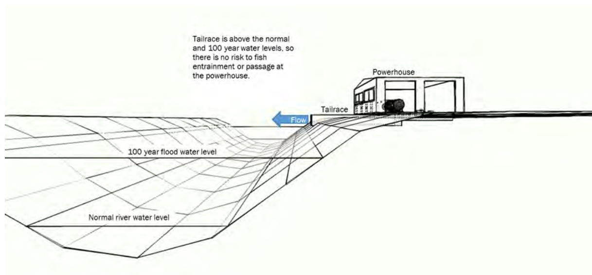
Figure 11 – Example of Pelton turbine powerhouse and tailrace above river water level
