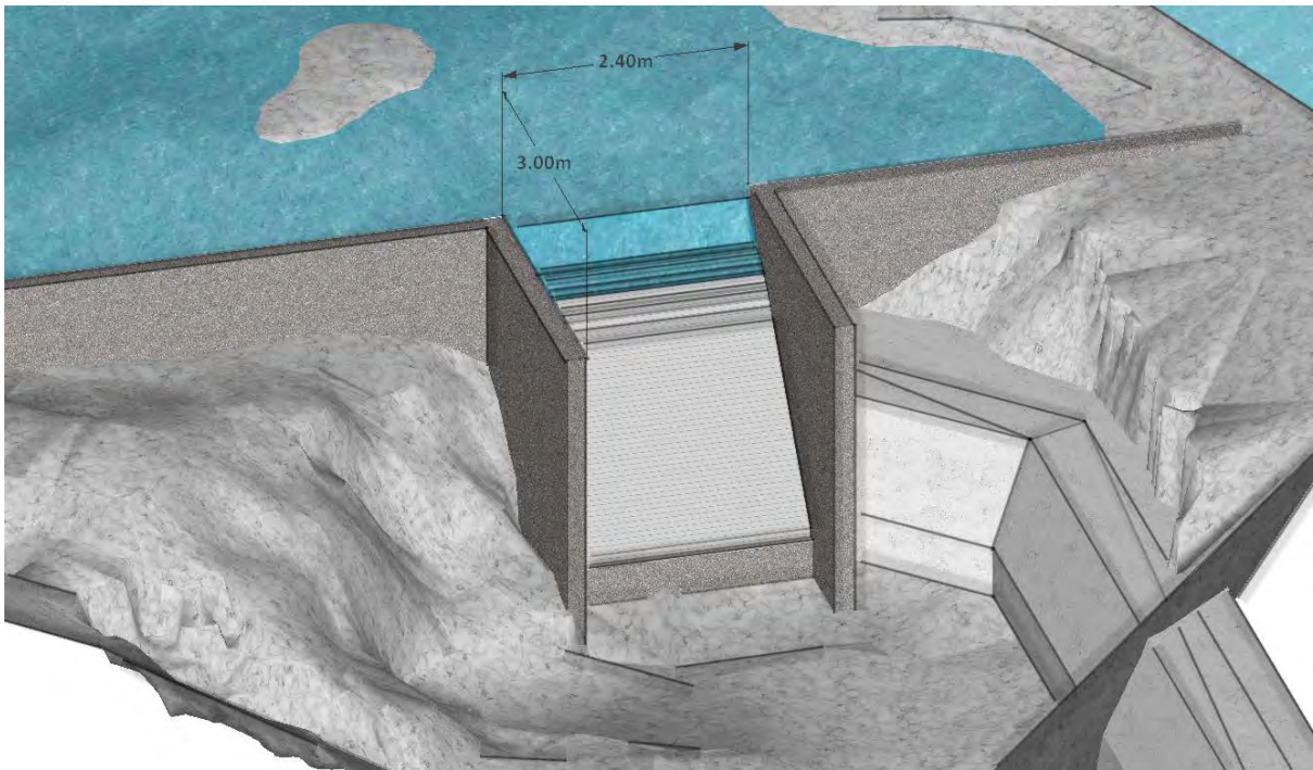
Figure 4 – Indicative dimensions of proposed Coanda intake and weir
