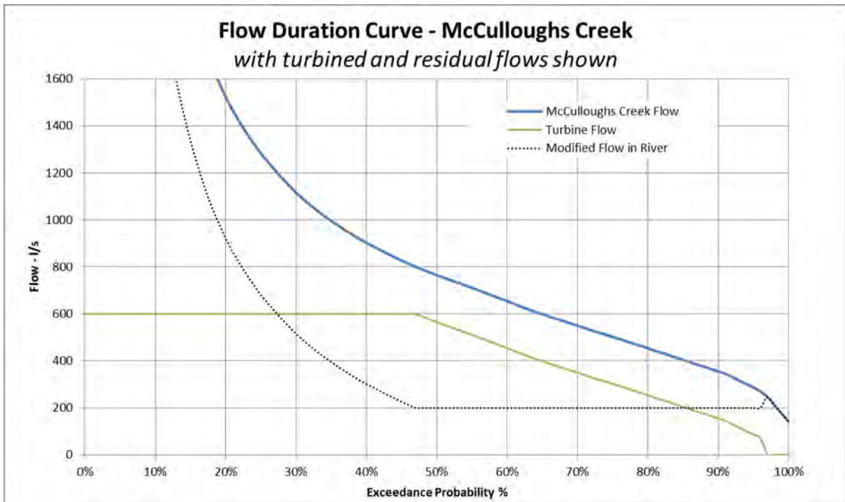
Figure 31 – Estimated flow duration curve at McCulloughs Creek intake
