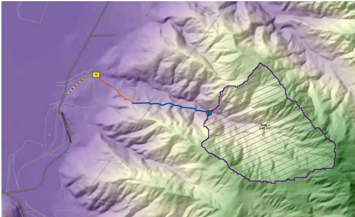
Figure 29 – Map showing McCulloughs Creek Hydropower Scheme and catchment at the intake site
