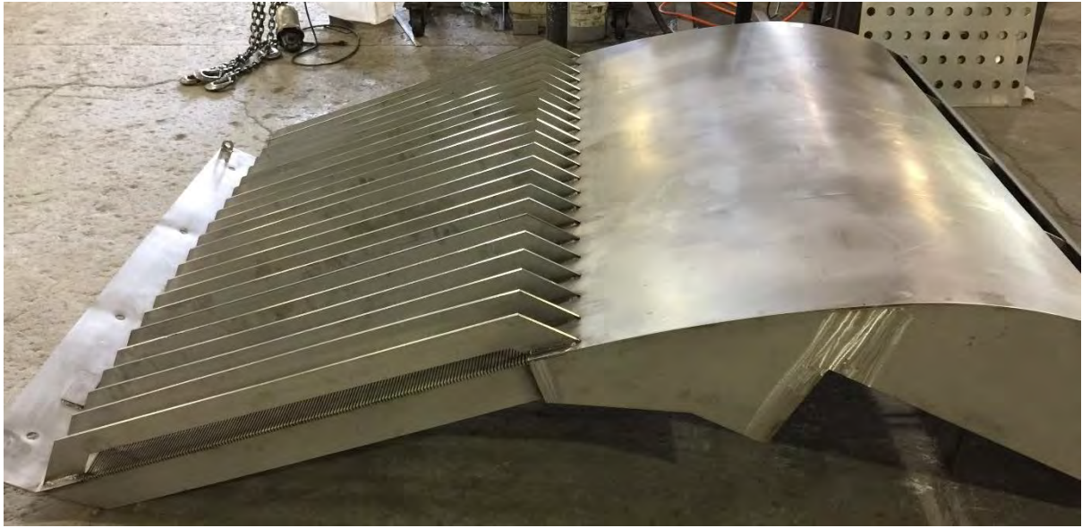
Figure 3 – Coanda screen with grizzly bars
