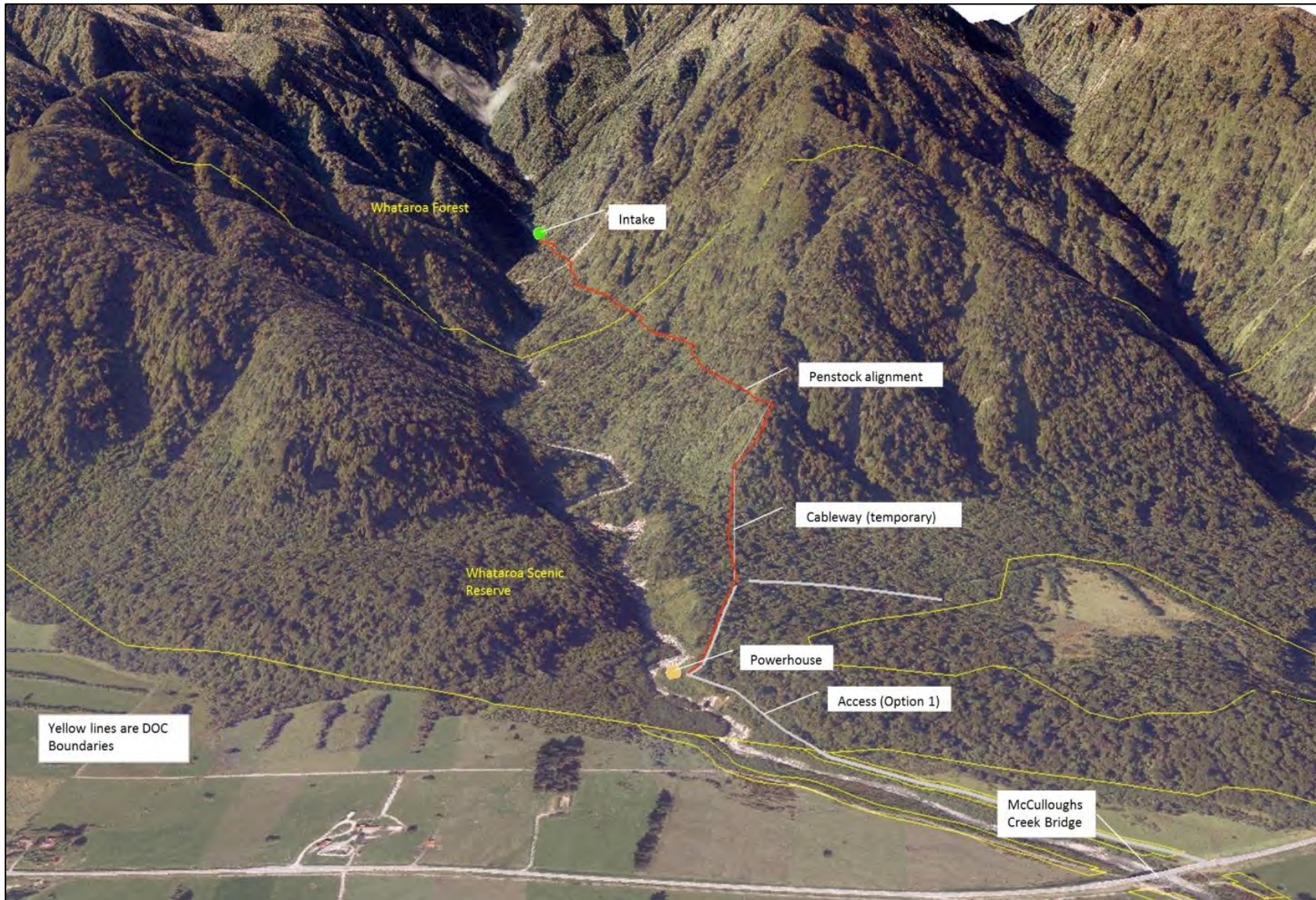
Figure 3: Overview of McCulloughs Creek and key components of the proposed hydropower project (map supplied by No.8 Ltd, August 2017).
