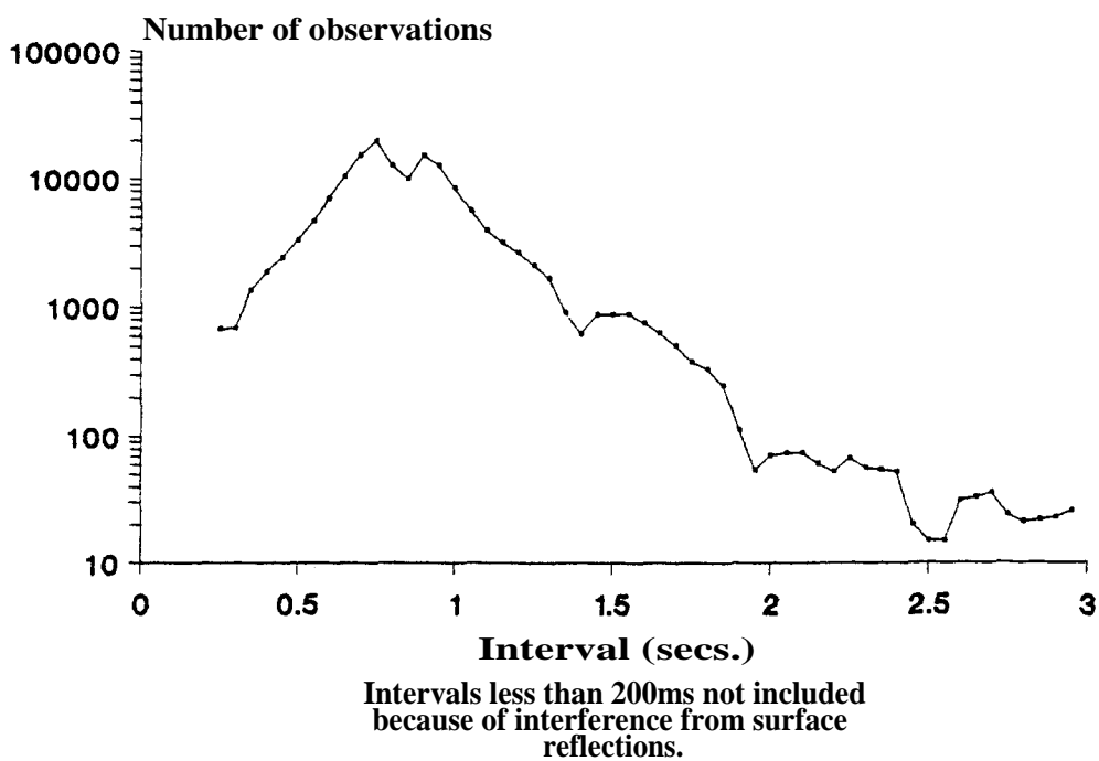
Figure 18 Frequency distribution of all inter-click intervals measured.
