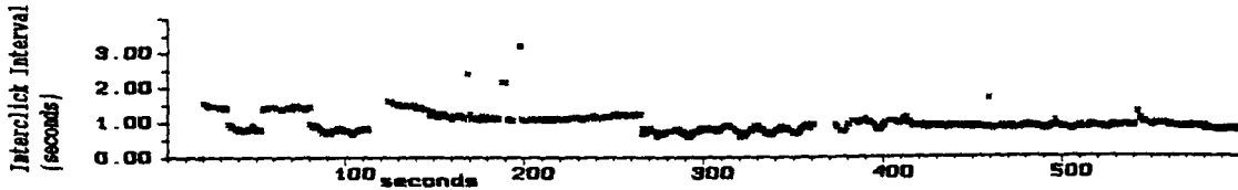
Figure 19 Examples showing plots of click intervals (s) against time in seconds since fluke up. Note that blow intervals tend to vary regularly. Horizontal triangles indicate creaks, and the length of triangle indicates duration of the creak
