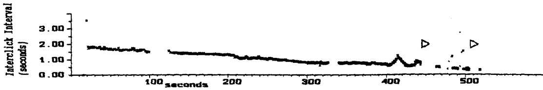
Figure 19 Examples showing plots of click intervals (s) against time in seconds since fluke up. Note that blow intervals tend to vary regularly. Horizontal triangles indicate creaks, and the length of triangle indicates duration of the creak
