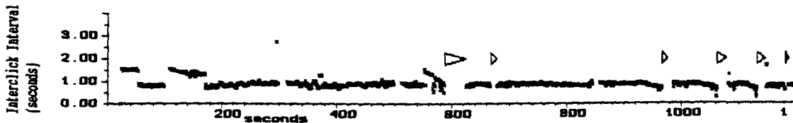
Figure 20 Example plots of inter-click intervals (s) against time since fluke-up showing the occurrence of sudden changes in click interval. Horizontal triangles indicate creaks, and the length of the triangle indicates duration of the creak.
