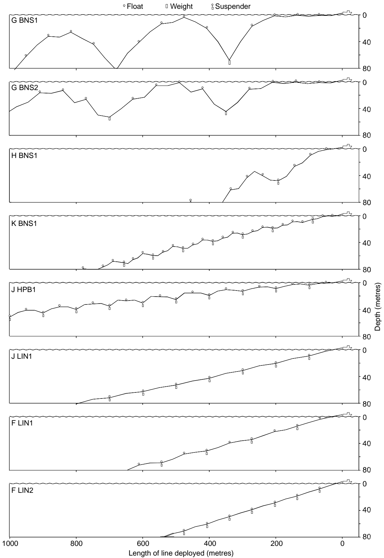
Figure 12. Composite profiles of longlines sinking behind vessels for the different line set ups shown in table 5. Labels show vessel identification, target species, set up number.
